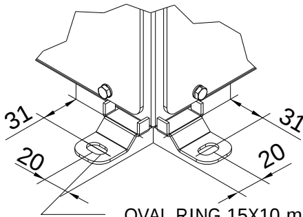
OVAL RING 15X10 mm
